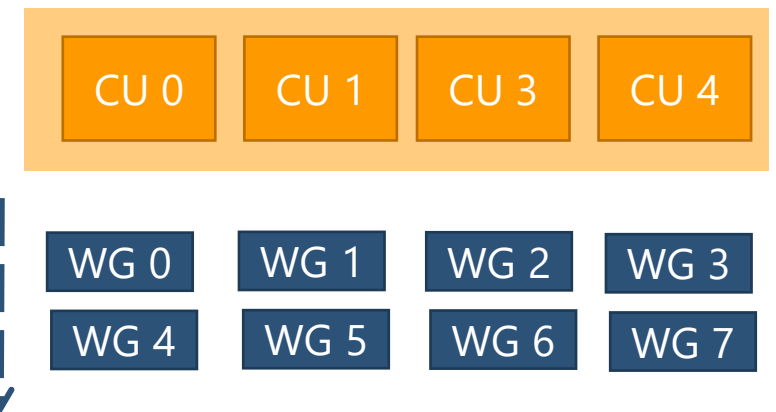
GPU with 4 CU
