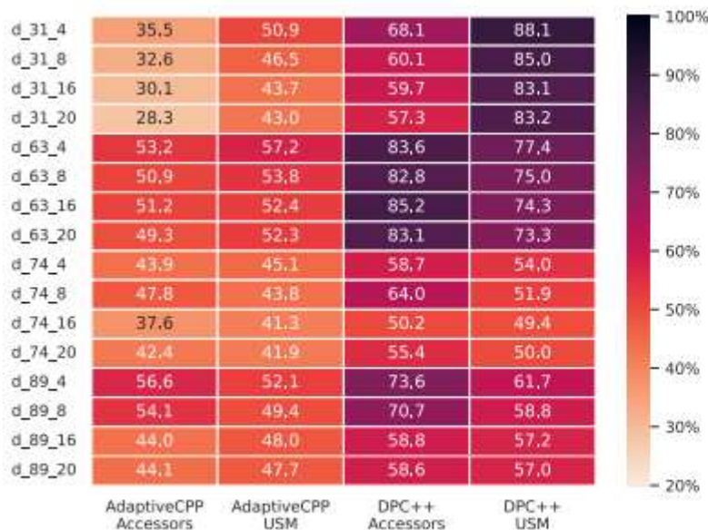
(a) LiGen Latency
