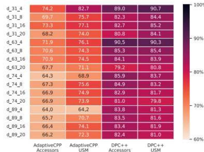
(b) LiGen Batch
